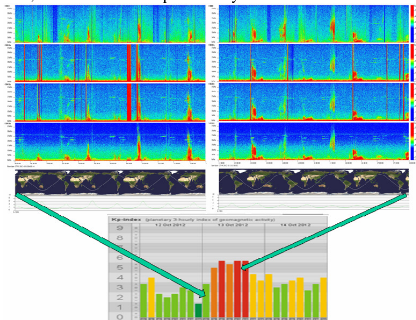
Figure. 7. "Chibis-M" 2012.10. 12-14. Top-down: E, Bx, By, Bz (see Fig. 5); projection of the “Chibis-M” orbit; L-parameter; Kp-index.
