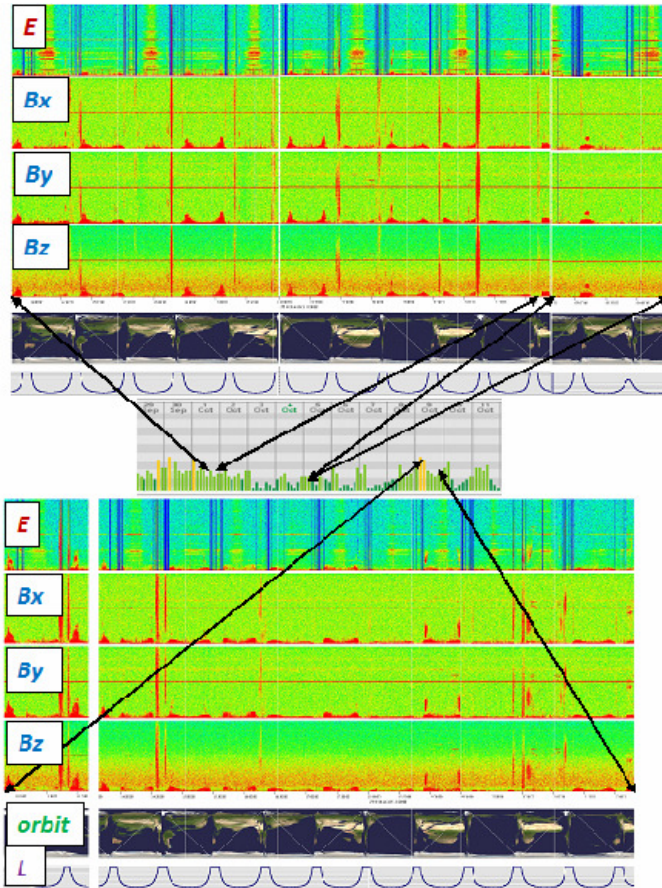
Figure 9. The experiment RELEC. Monitoring electromagnetic parameters (0.01-22kHz): the top row 2014/10/01 13:40-22:00 UT; the bottom row 2014/10/09 10:18-22:20 UT. Arrows highlighted the value of the Kp index (middle) at selected time intervals.
