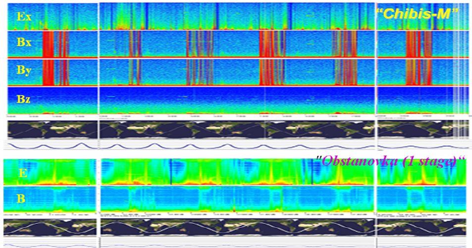
Figure. 6. Synchronous data "Chibis-M" and "Obstanovka the 1st stage" 2013.06.11 (UT+3) 10:00-20:00. Top-down: "Chibis-M": E, Bx, By, Bz – frequency 0.01-39kHz; "Obstanovka (1-st stage)": E, B – frequency 0.01-23kHz.
