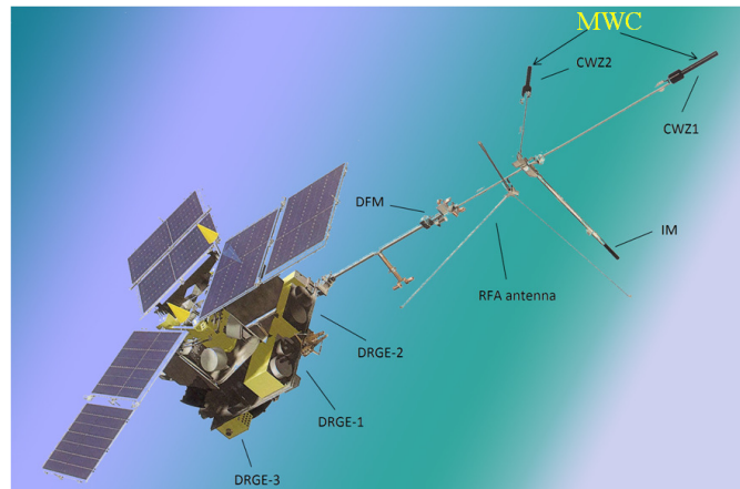
Figure 8. RELEC experiment on-board "Vernov" spacecraft: identical detectors of X- and gamma-rays of high temporal resolution (DRGE-1 and DRGE-2) detectors of energetic electrons and protons mounted along Cartesian frame (DRGE-3), ultraviolet TLE imager (MTEL), ultraviolet high time resolution detector (DUV), Magnetic Wave Complex (MWC: CWZ1, CWZ2, IM), RFA radio-frequency analyser.
