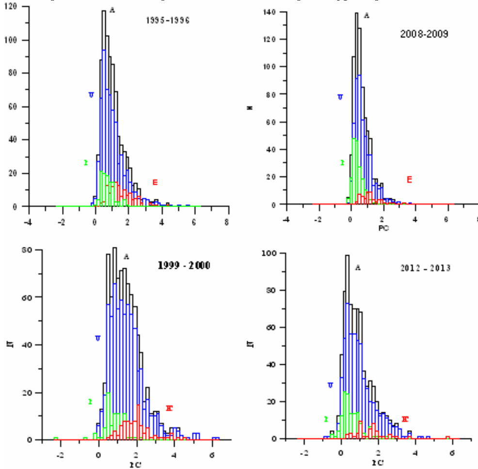
Fig. 2 PC index before substorm onsets for 1995-1996, 1999-2000 (left columns) and for 2008-2009, 2012-2013 (right columns)
