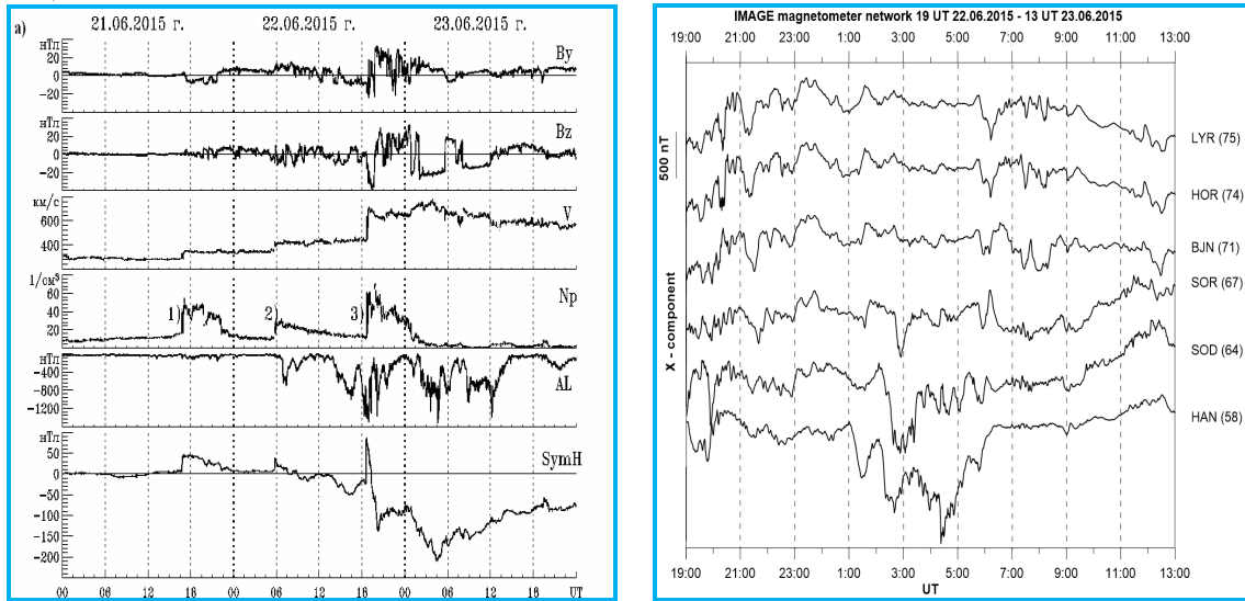
Fig.2. IMF and solar wind data and the AL and SymH indexes (left panel), magnetograms from selected IMAGE stations, geomagnetic latitudes are given in brackets.
