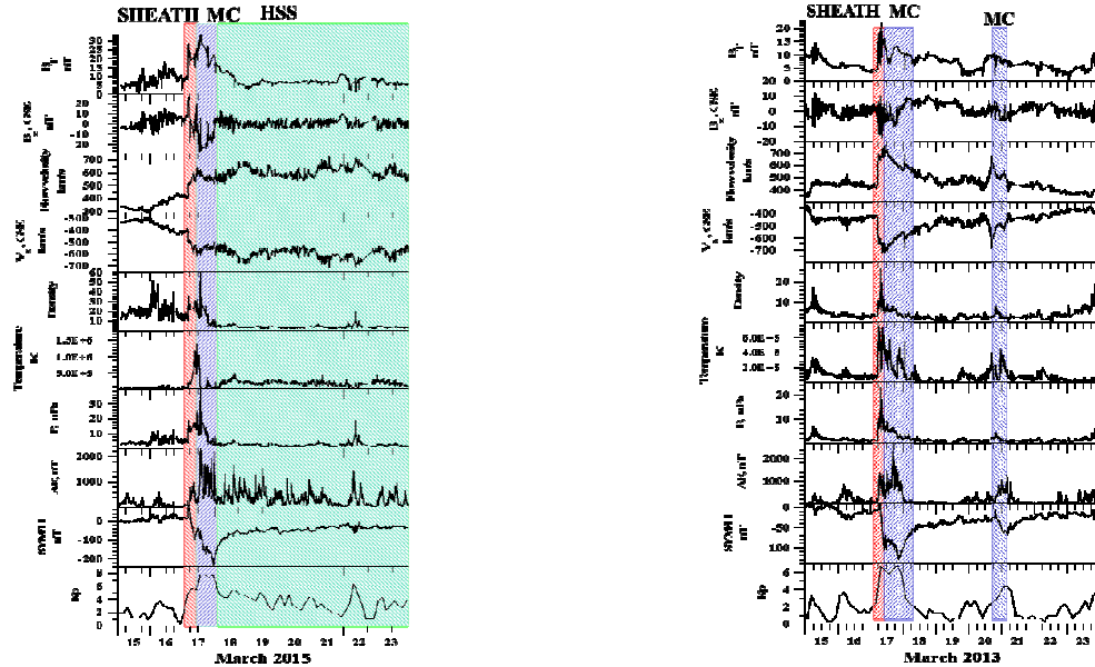
Figure. 1. The solar wind conditions taken from the OMNI database for the period 15–23 March 2015 (left panel) and 2013 (right panel). There some solar wind and IMF parameters, the AE, SYMN/H and Kp indices are presented. The solar wind magnetic cloud (MC), SHEATH and the high speed stream (HSS) regions are shown by shaded blue, red and green rectangles.
