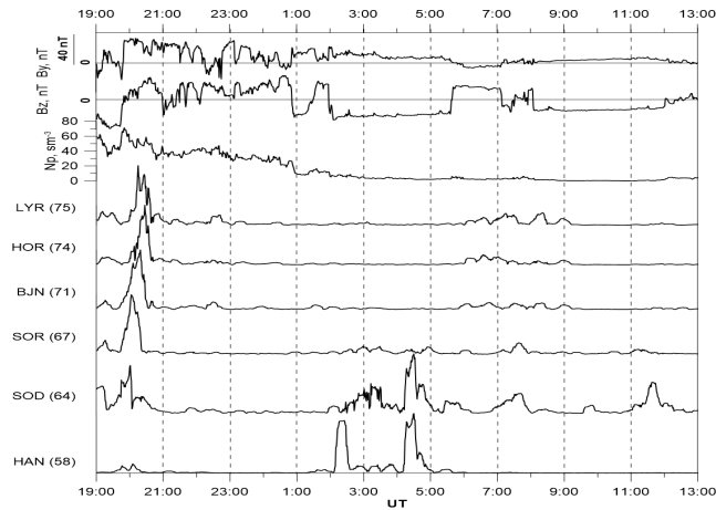
Fig.3. Results of Pi3 geomagnetic pulsation study.
