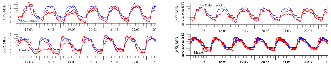
Figure 4. foF2 variations over Kaliningrad and Irkutsk according to the ionosonde data (circles) and model-derived results (lines) on March 17–23 (red color) comparing with the quiet geomagnetic conditions (blue color). Results for 2015 are presented at the left panel and for 2013 storm at the right panel.
