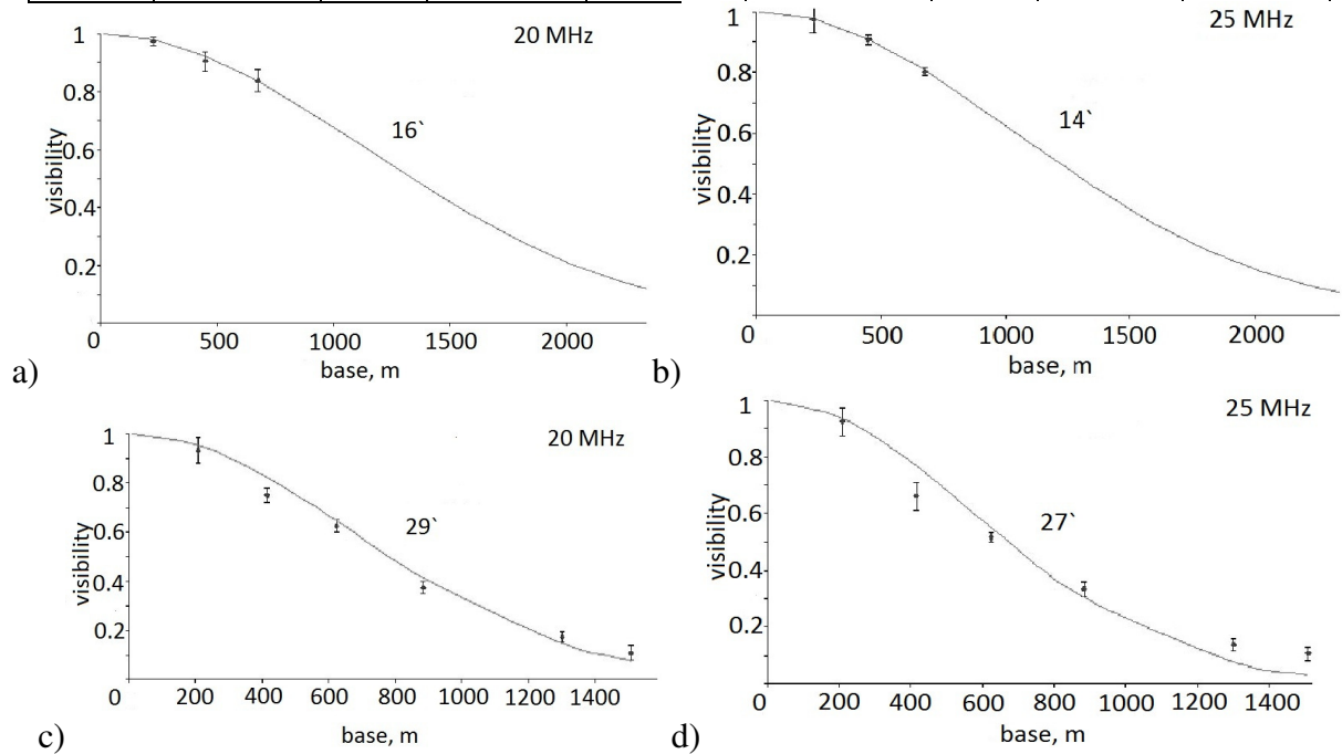
Figure 2. Visibility functions for type III bursts observed at 9:41 on May 29 (a,b) and at 6:59 on June 2 at frequencies 20 MHz and 25 MHz.
