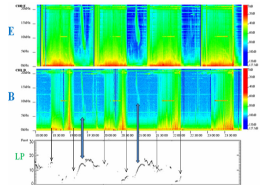
Figure 3. "Obstanovka (1 stage)". Monitoring electric E (1 st - upper panel) and magnetic B (2 nd ) components Data identical to Fig. 2. Bottom panel - synchronous potential data of the ISS outer surface by the device LP.
