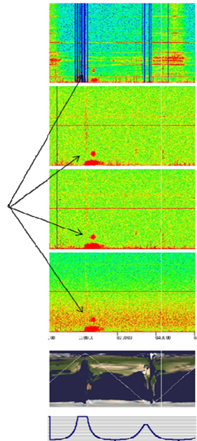
Figure 10. The experiment RELEC 2014/10/05 02:37-04:30 UT. A single short-term narrow-band radiation at frequency of ~5 kHz highlighted arrows
