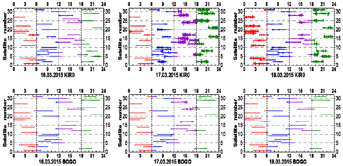
Fig.2. Development of TEC fluctuations at midlatitude BOGO and KIRO stations for quiet (16 March), storm (17 March) and recovery phase (18 March) days.
