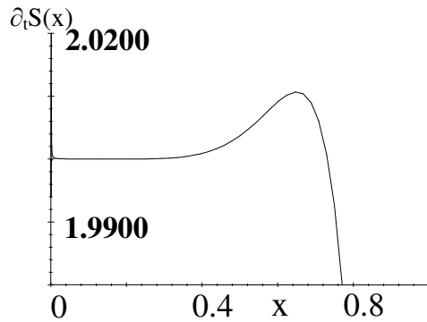
Fig.1a: Development of the gradient of entropy \partial_t S(x) over dimensionless radius of the disk x = r/r_{out} , ( r_{out}=103R_g ) in Cyg X-1.
