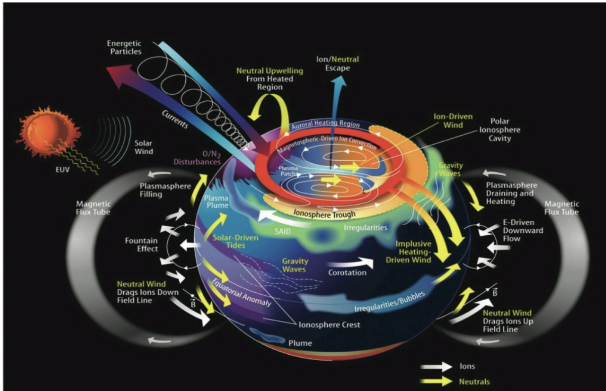
Figure 1. Schematic structure of the ionosphere.
